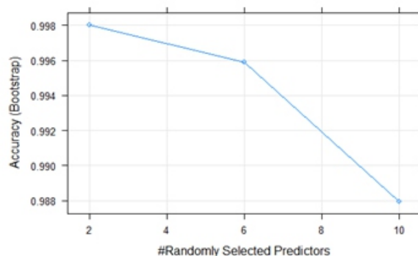
Figure 4- Accuracy of Randomly selected predictors
