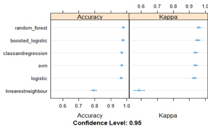
Figure 3- Comparison of the six models
