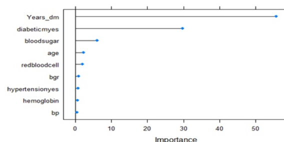
Figure 2- Listing of features
