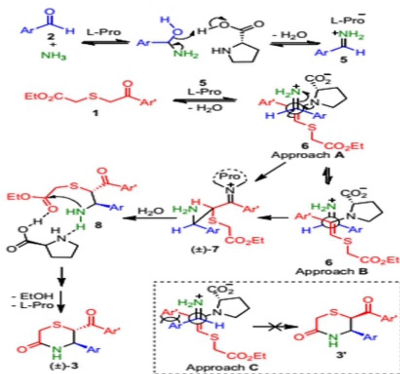
Scheme 2. Mechanistic proposal to explain the diastereoselective formation of compounds 3.
